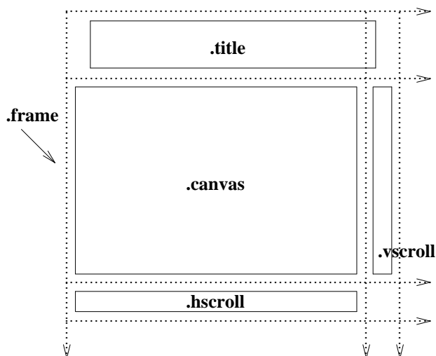
Figure 1. Example of Table Layout
